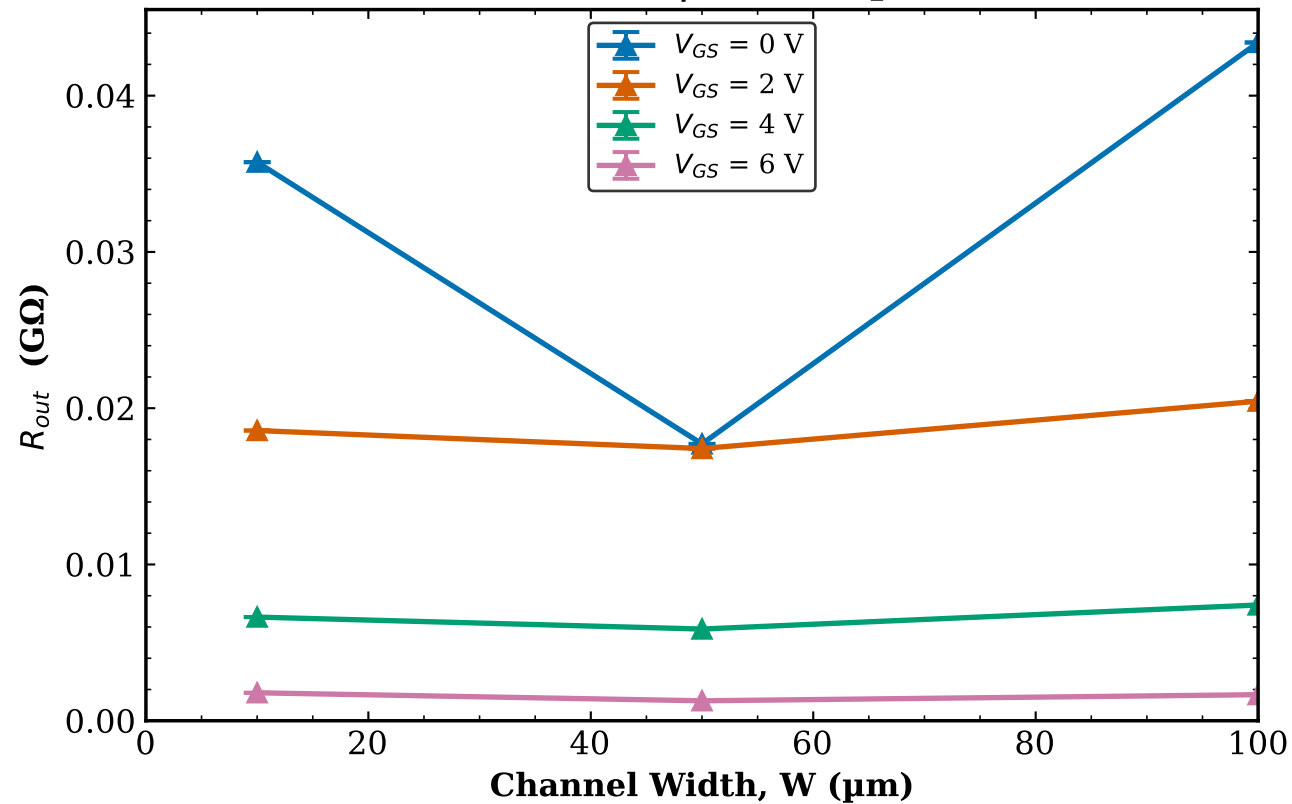
TFT3 Transistor 1 R_{out} vs W | L = 20\text{ }\mu\text{m}
